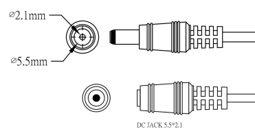
DC JACK 5.5*2.1
